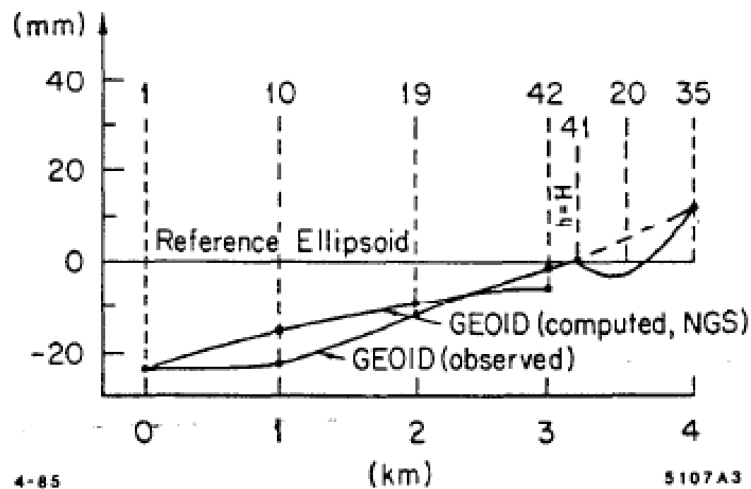
Figure 3 Geoid Profile
