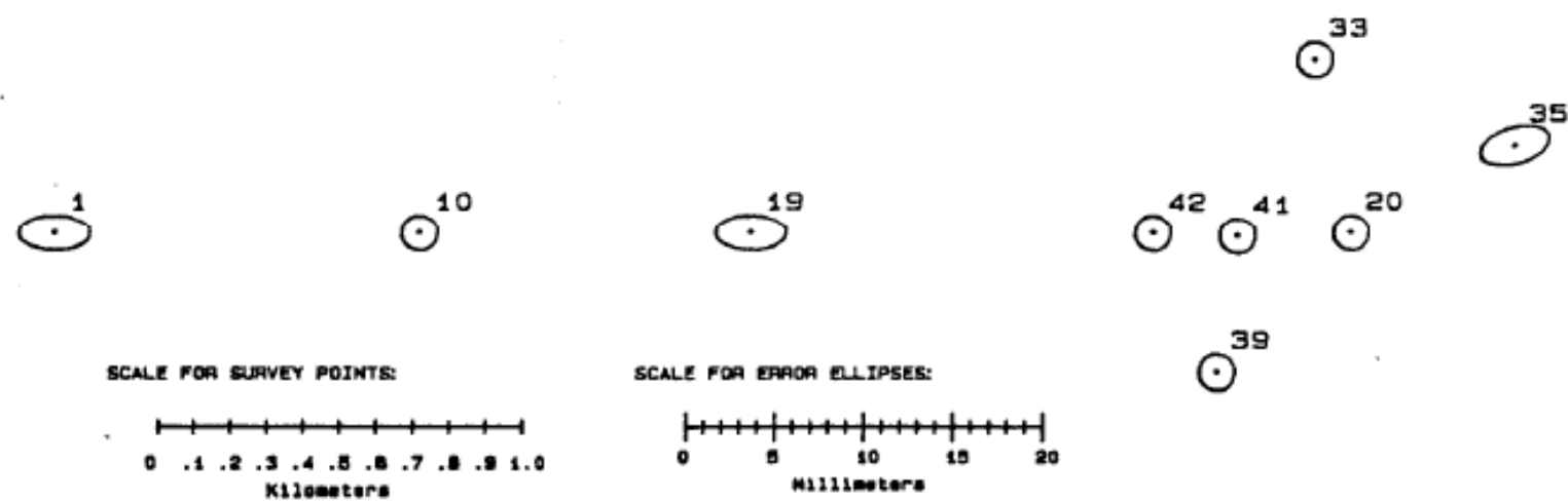
Figure 2 Error Ellipses from GPS Inner Constraint Solution
