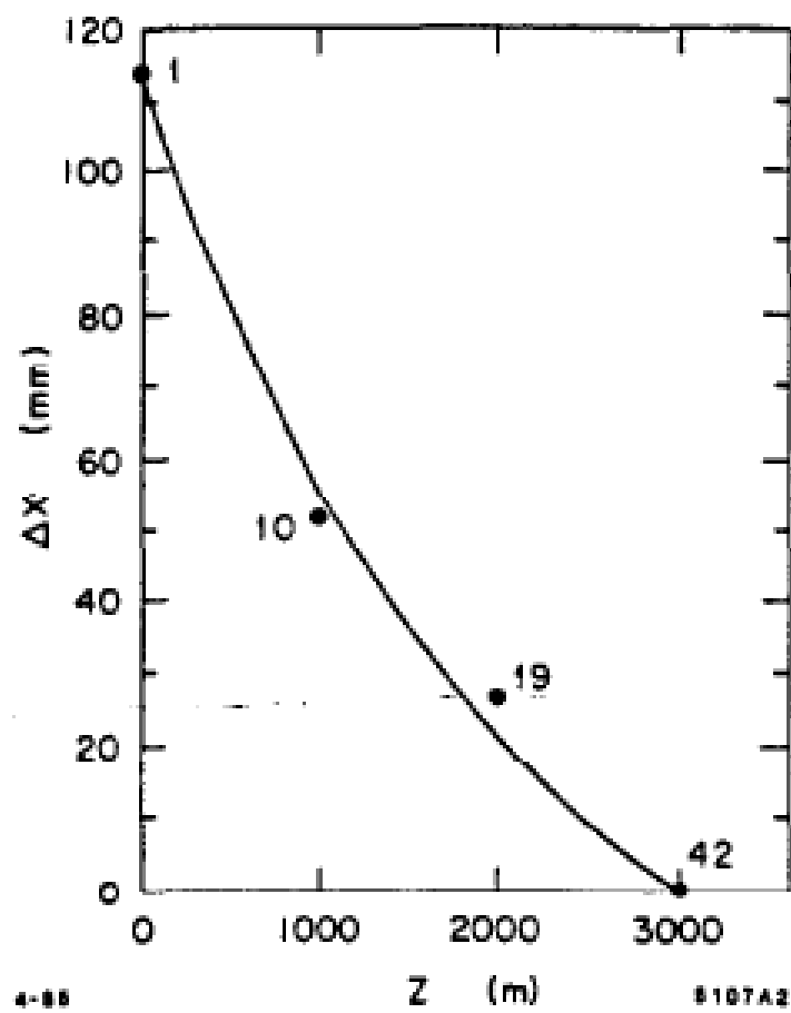
Figure 5 Linac Discrepancies
