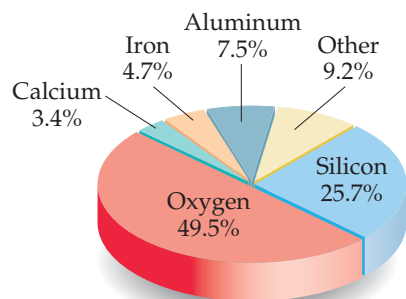
Earth's crust
