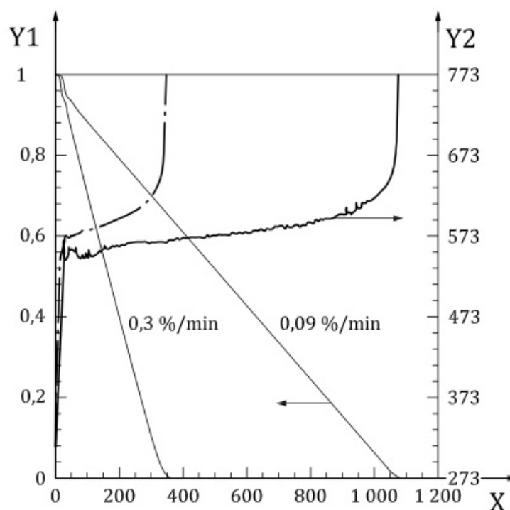
b) Example of sample mass controlled rate thermogravimetry (CRTG) measurements of PMMA
